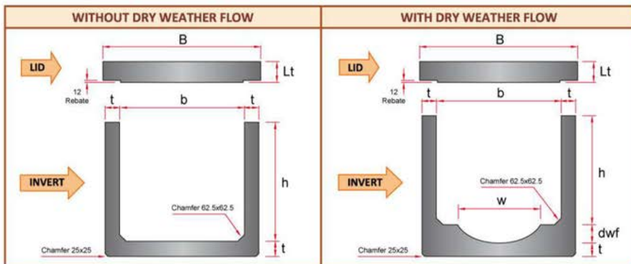
DETAILS OF OKA STANDARD SIZE BOX CULVERT
